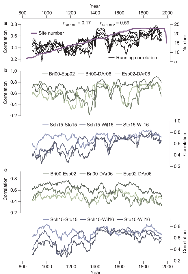
Fig. 6. Reconstruction co-variance. a , 100-running correlations among large-scale temperature reconstructions. Each black curve represents the mean derived from correlating one record against its five counterparts. The purple curve is the average number of site chronologies (or clusters) combined in the reconstructions from 831–1992. b , Running correlations between the early records (Bri00, Esp02, DAR06) in green and between the recently published records (Sch15, Sto15, Wil16) in blue. c , Same as in b , but for the first differenced records.
